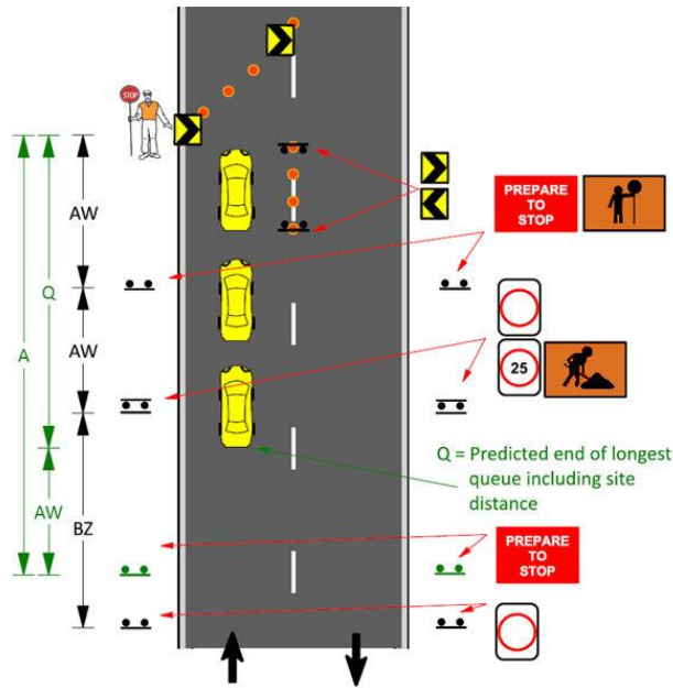
Figure 5.2: Avoiding end of queue collisions
